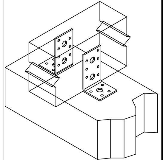
Installation for 2 brackets
